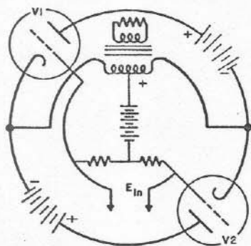
Fig. 5 — Simplified Diagram Circlotron Circuit
